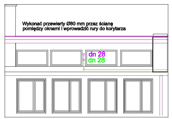
WIDOK "A"
